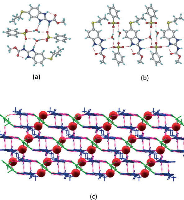
Fig. 3 (a) The bridging water molecules act as proton donors for the sulfonate and acceptors for \text{N}^+\text{-H} resulting in the ring network \text{R}_3^2(8) \text{R}_4^4(12)\text{R}_3^2(8) . (b) The sulfonate-water molecules are bonded via \text{N-H}\cdots\text{O}^- hydrogen bonds to ABZ. (c) Complete packing of cations, anions and water molecules.
