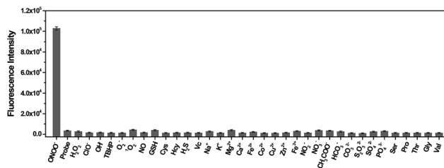
Fig. 1 Fluorescence response of TP-KA (1.0 \mu M) with various bioanalytes, including ONOO - (10.0 \mu M), H 2 O 2 (200 \mu M), other ROS and RNS (10.0 \mu M), GSH and Cys (5.0 mM), and other interfering substances (100 mM). The data were recorded after the incubation of TP-KA with various bioanalytes for 10 min at 37 ^{\circ} C in PBS buffer (50 mM, 7.4) with 1% DMSO. The values are the mean \pm s.d. for n = 3 . \lambda_{\text{ex}}/\lambda_{\text{em}} = 430/560 nm.
