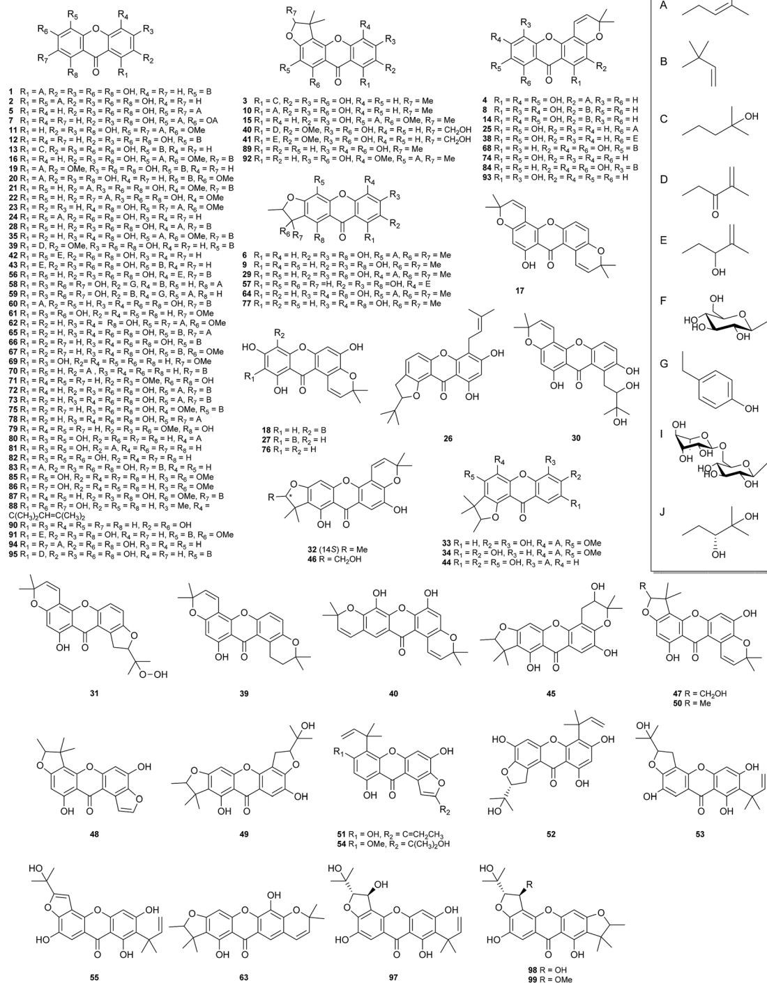
Fig. 2 Chemical structures of xanthones and flavonoids isolated from C. tricuspidata .
