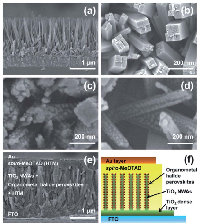
Fig. 17 Cross-sectional (a) and top (b) view SEM images of \text{TiO}_2 nanowire arrays (NWAs) synthesized on FTO substrates. SEM images of \text{CH}_3\text{NH}_3\text{PbI}_2\text{Br} (c) and \text{CH}_3\text{NH}_3\text{PbI}_3 (d) spin-coated on \text{TiO}_2 NWAs. (e) Cross-sectional SEM image of the \text{TiO}_2 NWAs/perovskite sensitizer/spiro-MeOTAD hybrid photovoltaic cell. (f) Schematic illustration of the hybrid solar cell.
