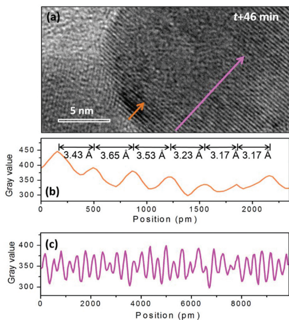
Fig. 5 (a) HRTEM image of the GdF 3 -NaGdF 4 interface at the irradiation time of 46 min. (b) and (c) Profiles of line scans along the GdF 3 -NaGdF 4 interface (orange arrow) and along the particle body of NaGdF 4 (111) (pink arrow).
