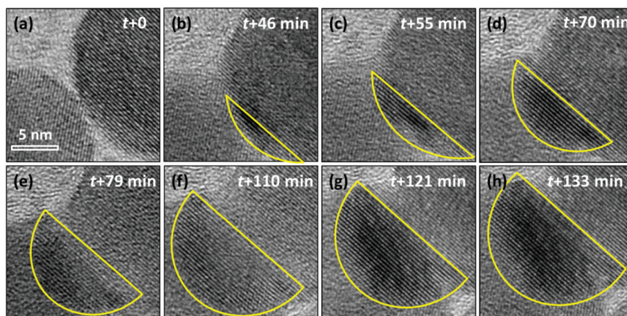
Fig. 4 (a–h) Time dependence of the in situ epitaxial growth of GdF 3 on NaGdF 4 at the interface induced by a focused electron beam with a current density of 40 pA cm -2 . The scale bar in all figures is 5 nm. GdF 3 layers are marked with yellow lines for a guide to the eye.
