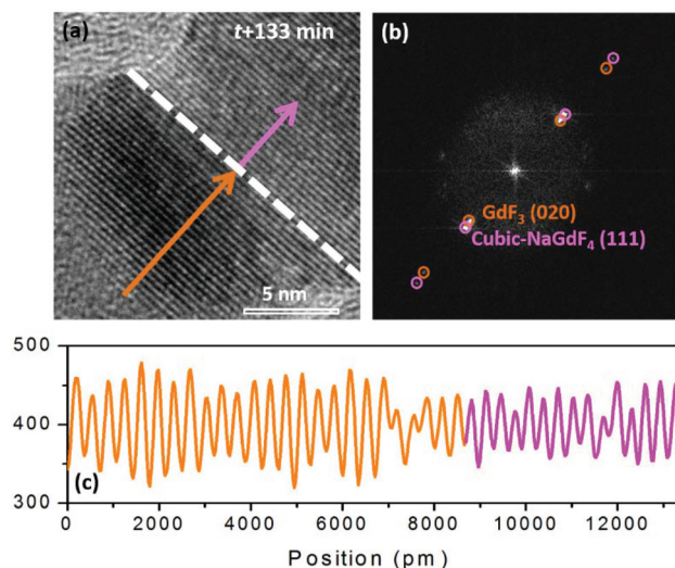
Fig. 6 (a) At t = 133 min, the HRTEM image shows a clear crystal interface between GdF 3 and NaGdF 4 indicated by a white dash line. (b) The associated FFT analysis definitely shows the co-existence of (111) of NaGdF 4 and (020) of GdF 3 with same direction. (c) Line scan indicated by the orange arrow and the pink arrow in (a) shows the averaged d -spacing for GdF 3 is 3.46 Å and that for NaGdF 4 is 3.17 Å, corresponding to the GdF 3 (020) plane and NaGdF 4 (111) plane.
