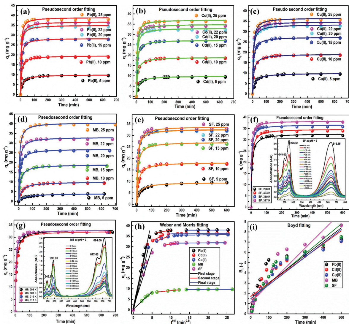
Fig. 9 Pseudo-second order kinetics plots for (a) Pb(II)-GGAAMAPA, (b) Cd(II)-GGAAMAPA and (c) Cu(II)-GGAAMAPA ( pH_i = 7 , T = 303 K and adsorbent dose = 0.05 g L -1 ), pseudo-second order kinetics plots for (d) MB-GGAAMAPA and (e) SF-GGAAMAPA ( pH_i = 10 , T = 303 K and adsorbent dose = 0.05 g L -1 ), pseudo-second order kinetics plots for (f) SF-GGAAMAPA and (g) MB-GGAAMAPA ( pH_i = 7 , Co = 30 ppm and adsorbent dose = 1 g L -1 , inset of (f), (g)) full scan kinetics data of SF and MB, respectively, (h) Weber and Morris fitting and (i) Boyd fitting of dyes and M(II).
