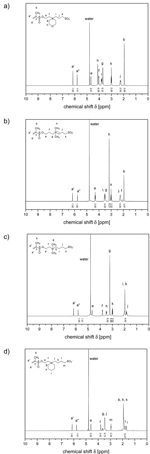
Fig. 2 ^1\text{H} NMR spectra of selected sulfobetaine methacrylate monomers \text{D}_2\text{O} (solvent signal at 4.78 ppm): ammoniopropansulfonates (a) 3 and (b) 4, and ammoniobutanesulfonates: (c) 5, and (d) 6.
