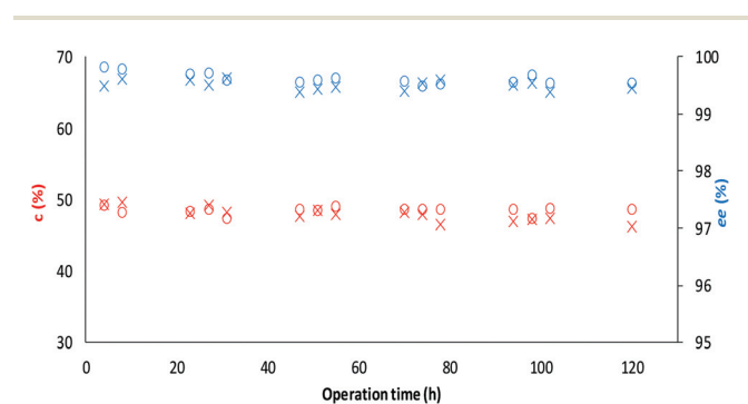
Fig. 8 Long term stability of the CaLB entrapped in the TDP sol-gel system in KR of the alcohol rac-1a ( c (%): x, ee_{(R)-2a} (%): x) and amine rac-3a ( c (%): o, ee_{(R)-4a} (%): o) in a continuous-flow reactor (60 °C, flow-rate of 0.1 mL min -1 ).
