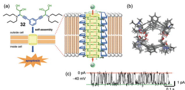
Fig. 7 (a) Schematic depicting of a self-assembly of bis-diol 32 in a lipid membrane. The Cl - selective channel that spans the membrane is proposed to consist of stacks of hydrogen bonded dimers of 32 2 . Transmembrane transport of chloride anions, which triggers apoptosis in a number of tested cell lines, is mediated by O–H...Cl - hydrogen bonds. (b) Top view of optimized structure of the anion channel formed by self-assembly of bis-diol 32 . (c) Single-channel current traces recorded at –40 mV holding potential in 1 M symmetrical KCl solution. The main conductance state is indicated by dotted lines. Reproduced from ref. 18. Copyright 2016, American Chemical Society.
