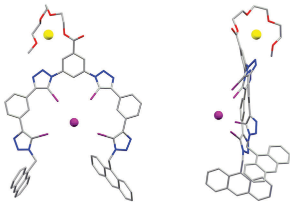
Fig. 3 X-ray crystal structure of 3b \cdot NaI showing the face-on (left) and side-on (right) view, visualising the folding of the receptor in a capped configuration.
