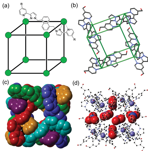
Fig. 1 The host cage [\text{Cd}_8\text{L}_{12}](\text{NO}_3)_{24} , H . (a) A sketch emphasising the cubic array of Cd(II) ions and the disposition of a bridging ligand L ( R = \text{CH}_2\text{OH} ); (b) a view of the complex cation from the crystal structure showing only four of the bridging ligands; (c) space-filling view of the complex cation with ligands coloured separately for clarity; (d) view of the complex emphasising the positions of some of the nitrate anions (shown space-filling) which occupy the portals on the faces of the cube. Additional figures showing the inclusion of dmf guest molecules and their interactions with the interior cage surface are in ESI.†
