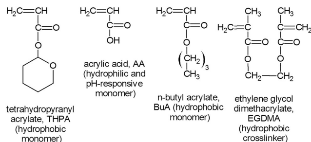
Fig. 2 Chemical structures of the monomers and crosslinker.
