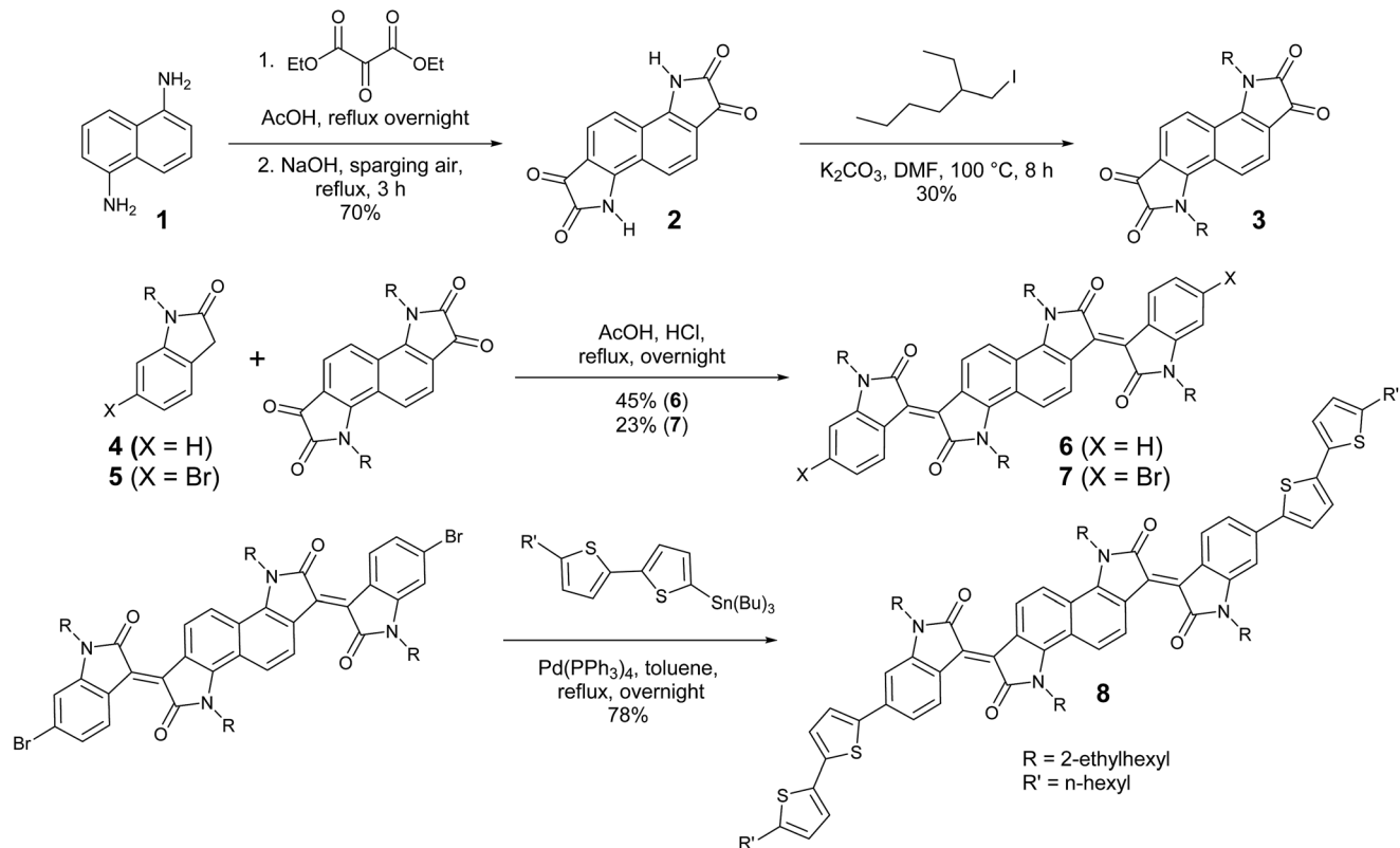
Scheme 1 Synthesis of bisoindigo (6) and bis(5'-hexyl-2,2'-bithienyl)-bisoinidigo (8).
