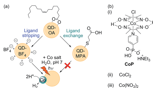
Fig. 1 (a) Schematic representation of the preparation and relative activity of the CdS QDs used in this study; (b) (i) structure of the molecular catalyst CoP, and (ii and iii) the two cobalt salts used as co-catalysts.
