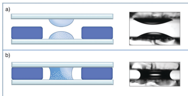
Fig. 3 Schematic representation (left) and photographs (right) of the measurement cell before (a) and after (b) the final assembly. (a) A drop of the colloidal suspension is deposited at the center of a glass slide while an identical drop of distilled water is deposited at the center of another slide. On the bottom slide, a gasket, obtained from a thin soft rubber sheet with a circular hole, is positioned. (b) The two drops are then aligned and put in contact. Immediately, a liquid bridge forms between the two slides and the diffusion process starts.
