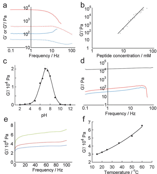
Fig. 6 Quantitative analysis of hydrogel mechanical properties using oscillatory shear rheometry. (a) Frequency dependence of standard hydrogel samples containing total peptide concentrations of 10 mM [ G' (—), G'' (---)] and 5 mM [ G' (—), G'' (---)]. (b) Plot showing the relationship between \log(G') and \log(\text{peptide concentration}) in hydrogels (linear curve fit to guide the eye). (c) Plot of G' versus hydrogel pH obtained under strain-sweep conditions, demonstrating that maximum stiffness is attained at around pH 7.2 (curve fit to guide the eye). (d) Frequency sweeps of standard hydrogel samples formed at pH 3 (—), 7 (—), and 11 (—). (e) Frequency sweeps of standard hydrogel samples separately formed at 20 °C (—), 37 °C (—) and 60 °C (—). (f) Plot of G' versus hydrogel temperature of a sealed sample, showing a non-linear relationship (curve fit to guide the eye).
