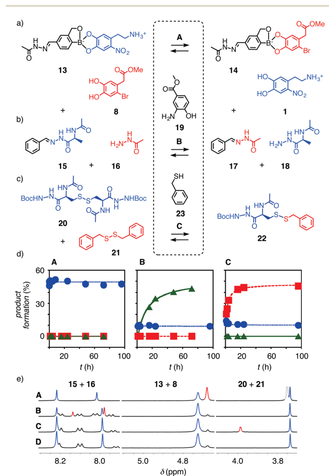
Fig. 3 (a–c) Exchange reactions used in this study to identify orthogonality under conditions A, B and C . (d) Exchange kinetics for boronate esters (●, 20 mM 13 , 22 mM 8 ) hydrazones (▲, 20 mM 15 , 20 mM 16 ) and disulfides (■, 20 mM 20 , 20 mM 21 ) under conditions A (DMSO- d 6 , 10% D 2 O, 2% DIPEA), B (1.0 mM 19 , 1.5 mM TFA in DMSO- d 6 ), and C (2.0 mM 22 , 2.0 mM TEA in DMSO- d 6 ). (e) Original data showing diagnostic peaks in 1 H NMR spectra in conditions A–C and D (DMSO- d 6 ) of 15, 20 and 13 (blue peaks) and their exchange products (red peaks). The signals at ~8.1 ppm disappear in conditions A due to H/D exchange.
