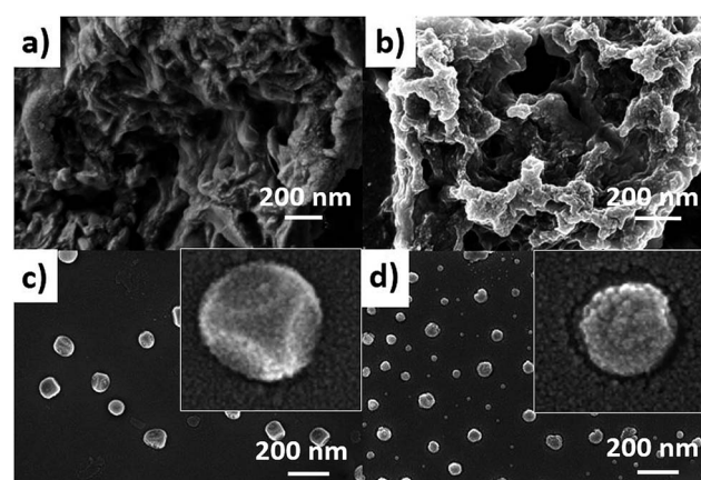
Fig. 2 SEM image of (a) hydrocalumite in solid state, (b) SOM 2 in solid state (c) hydrocalumite in dispersion, (d) SOM 2 in dispersion.
