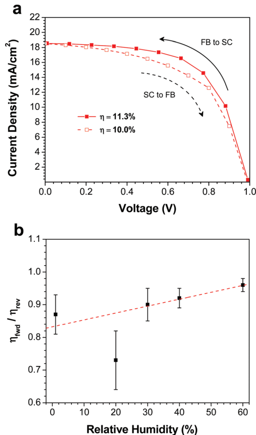
Fig. 5 (a) J-V curves measured at 0.1 \text{ V s}^{-1} for the best device prepared at 40% RH. (b) Ratio of PCEs determined from forward (SC-FB) and reverse (FB-SC) scans as a function of RH. The linear fit is a guide to the eye.
