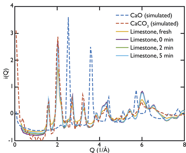
Fig. 6 Total scattering data of the limestone series compared to the corresponding calculated functions for \text{CaO} and \text{CaCO}_3 . The model PDF for \text{CaCO}_3 matches most features of the experimental data, confirming that this is the main phase contained in the samples.
