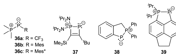
Fig. 6 Examples of zwitterionic phosphoniumphosphanides comprising bonding motif E.
