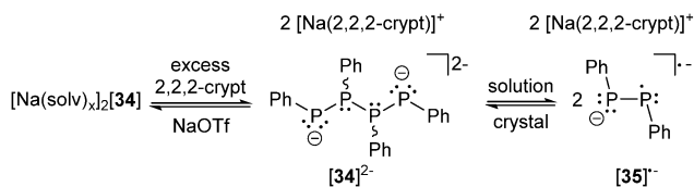
Scheme 13 The sodium ions of [Na(solvent)_x]_2[34] can be sequestered by 2,2,2-crypt. In solution the product splits into two radical anions [35]^{\bullet-} . Only one resonance structure of [35]^{\bullet-} shown.
