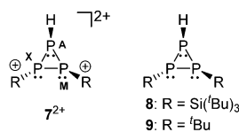
Fig. 2 Substituent arrangement in cyclo -triphsphanes 7^{2+} , 8 and 9 .
