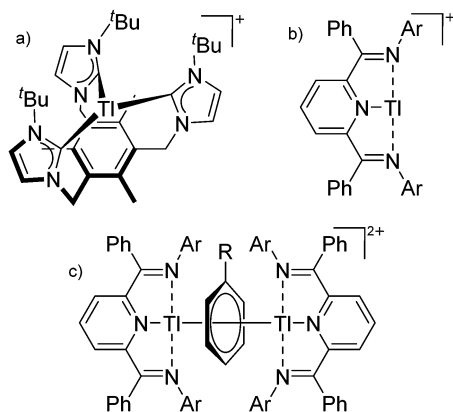
Fig. 27 Both the (a) [Tl(timtm-bu)]^+ and (b) [ArN=CPh]_2(NC_5H_5)Tl]^+ complexes derive from Tl^+[OTf]^- and are synthesized via complexation reactions of the corresponding ligands. In addition, the inverted sandwich structure (c) [ArN=CPh]_2(NC_5H_5)Tl]_2(\mu-\eta^6-C_6H_5R)]^{2+} ( Ar = 2,6-Et_2C_6H_3 , 2,5-tBu_2C_6H_3 ; R = H, Me ) was isolated.
