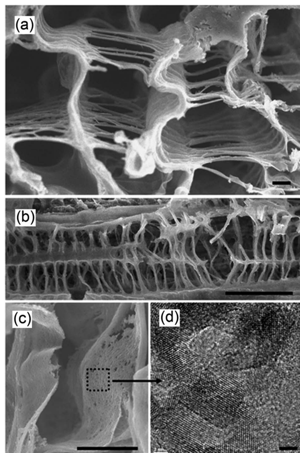
Fig. 15 FE-SEM images showing (a) the cross section of the porous network architecture of \text{SrTiO}_3 (scale bar, 1 \mu\text{m} ) (b) cross section of the porous network axially (scale bar, 10 \mu\text{m} ), (c) magnified image of the wall of the network (scale bar, 1 \mu\text{m} ) and (d) TEM image showing the mesoporous structure of \text{SrTiO}_3 (scale bar, 2 nm). Reprinted by permission from Macmillan Publishers Ltd ref. 158, copyright 2013.
