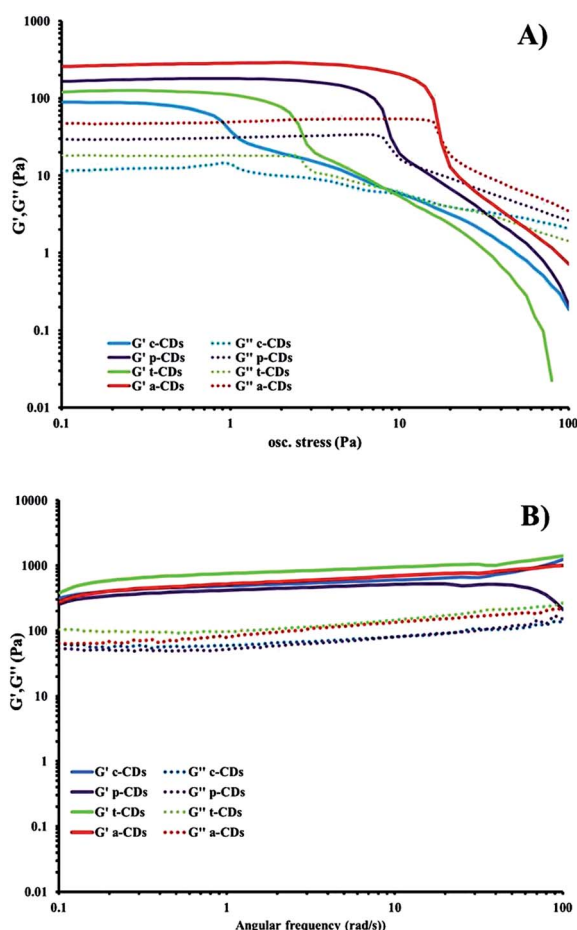
Fig. 5 (a) Stress sweep and (b) frequency-sweep rheology of dilute ionic-liquid CD–gel hybrid materials of composition 1 wt% 1a in 500 \mu\text{L} of CD solution at 1 \text{ mg mL}^{-1} containing 2% BMIM-BF 4 .
