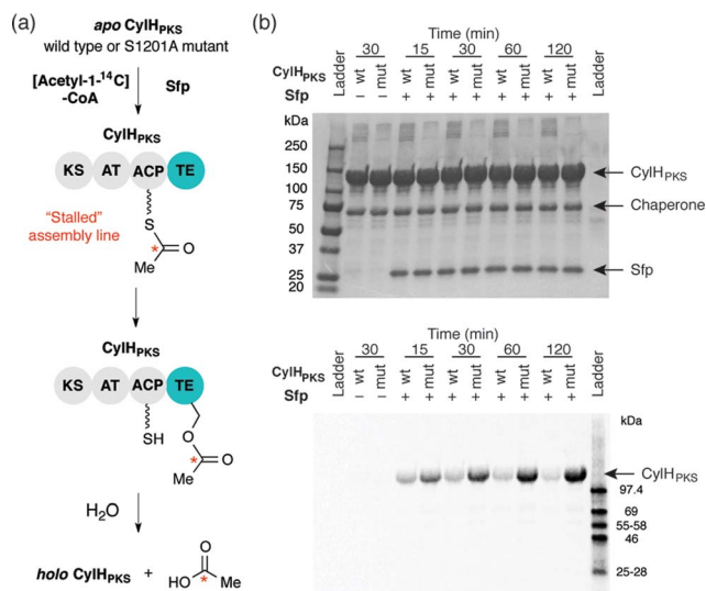
Fig. 5 The CylH TE domain hydrolyzes an acetyl-ACP intermediate on a stalled version of CyH. (a) Design of a gel autoradiography assay to assess the ability of CylH PKS to hydrolyze an [ 14 C]-ACP intermediate. (b) Autoradiogram of these reaction time course for hydrolysis of 14 C-acetyl-ACP-loaded wild type CylH PKS and the CylH PKS -S1201A mutant (top image = Coomassie stained gel, bottom = autoradiogram).
