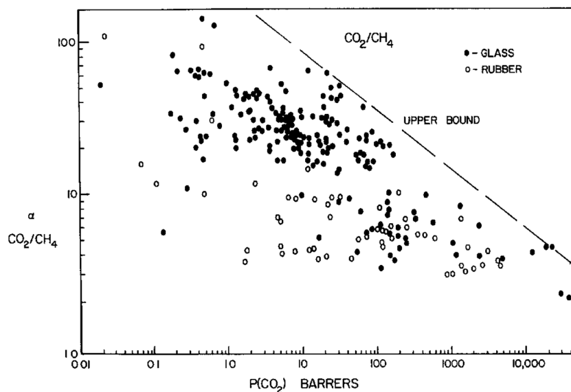
Fig. 7 Literature data for CO 2 /CH 4 ideal selectivity versus CO 2 permeability (1991).
