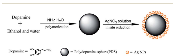
Fig. 1 Schematic illustration of the procedure for fabricating poly-dopamine sub-micrometer spheres loaded with silver nanoparticles (Ag@PDS).
