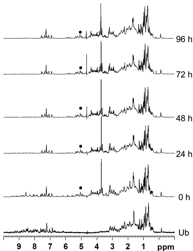
Fig. 3 1 H NMR spectra of the mixture Ub/[1] 6+ (molar ratio 1:10, D 2 O, 37 °C) recorded between 0 h and 96 h. The 1 H NMR spectrum of free ubiquitin is shown as reference at the bottom. The p -cymene resonances of the metallaprism are labelled by (■).
