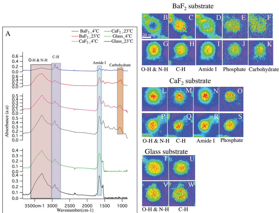
Fig. 1 (A) Total absorbance raw average spectra of the large-diameter DRG neuron on each IR optical substrate and thermal condition are shown. (B–K) Chemical images derived from large neurons plated on BaF 2 substrate and cultured in 4 °C (B–F) and 23 °C (G–K) for O–H & N–H group (B, G), hydrocarbon (C, H), Amide I (D, I), PO 2- asymmetric stretching of phosphate (E, J) and C–C and C–O–C stretching of carbon (F, K). (L–S) Chemical images derived from large neurons plated on CaF 2 substrate and cultured in 4 °C (L–O) and 23 °C (P–S) for O–H group (L, P), hydrocarbon (M, Q), Amide I (N, R) and PO 2- asymmetric stretching of phosphate (O, S). (T–W) Chemical images generated from respective neuron plated on glass substrate and cultured in 4 °C (T–U) and 23 °C (V–W). Scale bar in (B) represents 20 μm and applied to all images.
