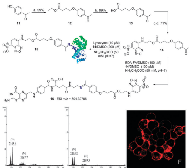
Scheme 5 (a) Ethyl 4-bromobutyrate, K_2CO_3 , NaI, acetone, reflux, 20 h; (b) TFA, H_2O , 90^\circ C , 3 h; (c) DMAP, EDC; DCM, 0^\circ C , 1 h; (d). NBDNH(CH _2 ) _2 OH, DCM, rt, 5 h. UV spectrum: see ESI† for compound 14 . Reaction of lysozyme (10 \mu M) with 14 (200 \mu M) in acetate buffer (50 mM, pH 7) at room temperature. Zoom of the (7+) charge state of the ESI-FTICR-MS spectra after 30 min and 2 h of reaction. Image F shows NCI-H460 treated with compound 16 . Incubation and imaging conditions are likewise described in Scheme 3.
