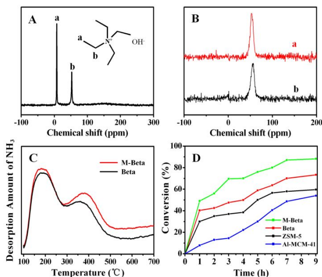
Fig. 3 (A) Solid-state ^{13}\text{C} NMR spectrum of uncalcined M-Beta. (B) Solid-state ^{27}\text{Al} NMR spectra of (a) uncalcined and (b) calcined M-Beta. (C) TPD- \text{NH}_3 curve of H form (red) M-Beta and (black) conventional Beta zeolite. (D) Performance comparison of M-Beta and conventional porous catalysts in the aldol condensation of benzaldehyde with n-butyl alcohol.
