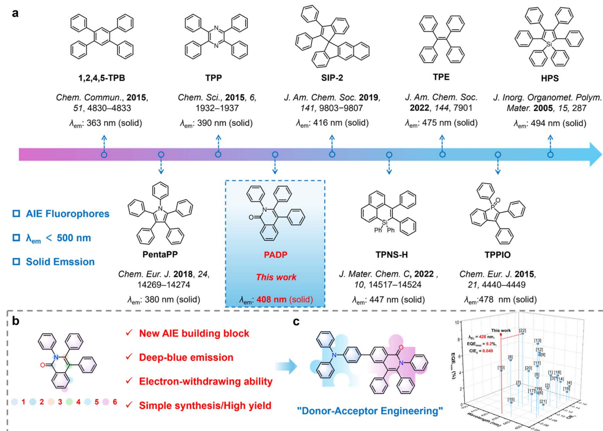
Fig. 1 (a) The main fluorescent molecules with AIE properties ( \lambda_{em} < 500 nm). (b) Molecular PADP and the sequence of naming its sites. (c) Molecular PADP-TPA; and \lambda_{EL} -CIE x -CIE y -EQE m summary data of deep-blue ( \lambda_{EL} \leq 450 nm) AIE fluorescent materials applied to OLEDs.
