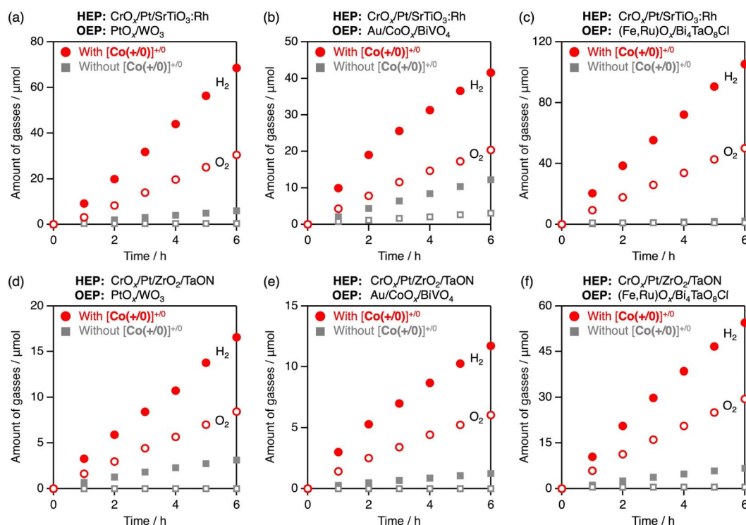
Fig. 8 Time courses of H 2 and O 2 evolution through Z-scheme water splitting in an aqueous solution (pH 3.5, 70 mL) in the presence or absence of [Co(+0)] +/0 (0.3 mM) as an electron mediator using the combination of (a) CrO x /Pt/SrTiO 3 :Rh–PtO x /WO 3 , (b) CrO x /Pt/SrTiO 3 :Rh–Au/CoO x /BiVO 4 , (c) CrO x /Pt/SrTiO 3 :Rh–(Fe,Ru)O x /Bi 4 TaO 8 Cl, (d) CrO x /Pt/ZrO 2 /TaON–PtO x /WO 3 , (e) CrO x /Pt/ZrO 2 /TaON–Au/CoO x /BiVO 4 , and (f) CrO x /Pt/ZrO 2 /TaON–(Fe,Ru)O x /Bi 4 TaO 8 Cl (each 70 mg) under visible light irradiation ( \lambda = 430 nm).
