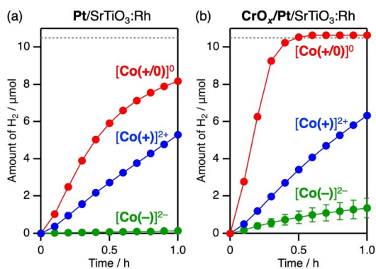
Fig. 3 Time courses of \text{H}_2 evolution using (a) Pt- or (b) \text{CrO}_x/\text{Pt} -loaded \text{SrTiO}_3\text{:Rh} (10 mg) in an aqueous solution (70 mL, pH 3.5) containing [\text{Co}(+)/]^{2+} , [\text{Co}(+/0)]^{+/0} , or [\text{Co}(-)]^{2-} (0.3 mM each) as an electron donor under visible-light irradiation ( \lambda = 430 nm). The broken lines show the upper limit of \text{H}_2 evolution expected from the amount of \text{Co}^{\text{II}} species added to the solutions.
