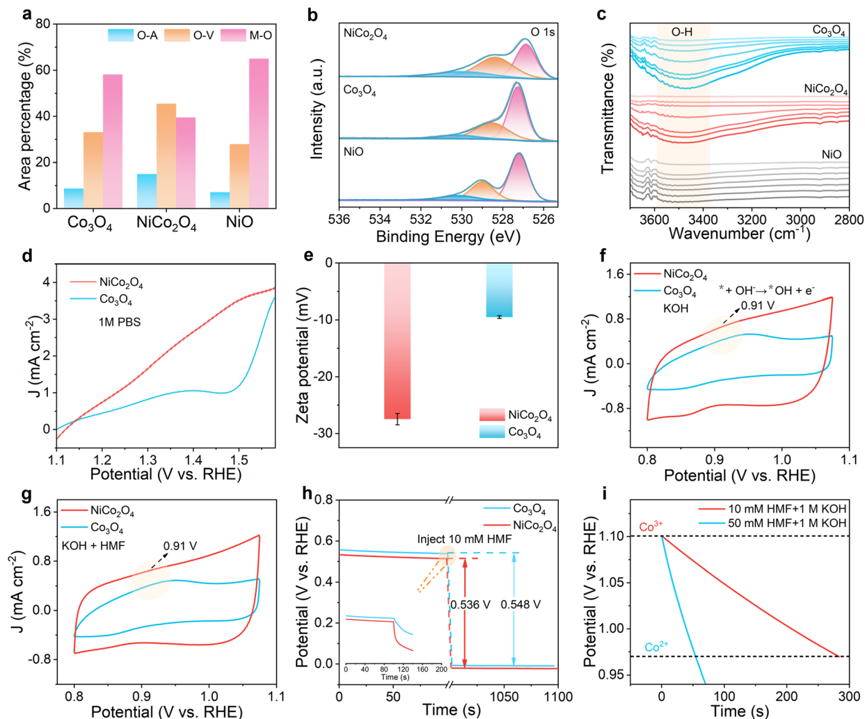
Fig. 3 (a) Relative content of oxygen vacancies, M-O, and adsorbed oxygen groups in the above samples. (b) High-resolution O 1s XPS spectra of \text{NiO} , \text{Co}_3\text{O}_4 and \text{NiCo}_2\text{O}_4 . (c) The in-situ FTIR spectra of \text{NiO} , \text{Co}_3\text{O}_4 and \text{NiCo}_2\text{O}_4 samples recorded at 1.5 V vs. RHE for 30 min in the HMFOR. (d) LSV curves of the \text{Co}_3\text{O}_4 and \text{NiCo}_2\text{O}_4 samples in 1 M PBS solution. (e) Zeta potential of the \text{Co}_3\text{O}_4 and \text{NiCo}_2\text{O}_4 samples. CV curves of the \text{Co}_3\text{O}_4 and \text{NiCo}_2\text{O}_4 samples in (f) KOH and (g) KOH + HMF solution. (h) The OCP of the \text{Co}_3\text{O}_4 and \text{NiCo}_2\text{O}_4 samples in 1 M KOH solution before and after HMF was injected. (i) \text{Co}^{3+} obliteration time test for \text{NiCo}_2\text{O}_4 .
