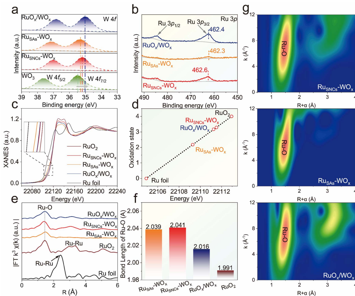
Fig. 2 (a) W 4f core level XPS spectra of \text{Ru}_{\text{SAs}}-\text{WO}_x , \text{Ru}_{\text{SNCs}}-\text{WO}_x , \text{RuO}_x/\text{WO}_x and \text{WO}_3 . (b) Ru 3p core level XPS spectra of \text{Ru}_{\text{SAs}}-\text{WO}_x , \text{Ru}_{\text{SNCs}}-\text{WO}_x and \text{RuO}_x/\text{WO}_x . (c) XANES spectra at the Ru K-edge of \text{Ru}_{\text{SAs}}-\text{WO}_x , \text{Ru}_{\text{SNCs}}-\text{WO}_x , \text{RuO}_x/\text{WO}_x , Ru foil and \text{RuO}_2 . (d) Oxidation states of various ruthenium species derived from Ru K-edge XANES. (e) FT-EXAFS of \text{Ru}_{\text{SAs}}-\text{WO}_x , \text{Ru}_{\text{SNCs}}-\text{WO}_x , \text{RuO}_x/\text{WO}_x , Ru foil and \text{RuO}_2 . (f) The fitted Ru–M bond length data of \text{Ru}_{\text{SAs}}-\text{WO}_x , \text{Ru}_{\text{SNCs}}-\text{WO}_x , \text{RuO}_x/\text{WO}_x and \text{RuO}_2 . (g) Wavelet transform of Ru K-edge EXAFS data of \text{Ru}_{\text{SAs}}-\text{WO}_x , \text{Ru}_{\text{SNCs}}-\text{WO}_x and \text{RuO}_x/\text{WO}_x .
