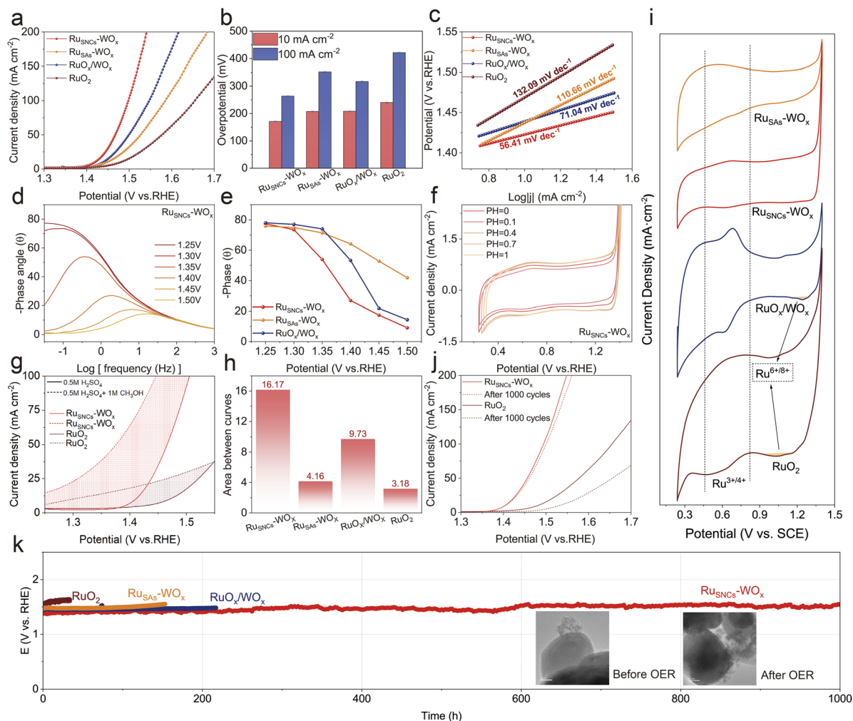
Fig. 4 (a) LSV curves of Ru SAS -WO x , Ru SNCs -WO x , RuO x /WO x and RuO 2 in 0.5 M H 2 SO 4 solution. (b) Comparison of overpotentials at a current density of 10 mA cm -2 and 100 mA cm -2 . (c) Corresponding Tafel plots according to the LSV curves in (a). (d) Bode phase plots of Ru SNCs -WO x at different voltages. (e) Summarized phase peak angles of Ru SAS -WO x , Ru SNCs -WO x , RuO x /WO x and RuO 2 at 1.25–1.50 V. (f) pH independent CV analysis of redox peaks of Ru SNCs -WO x measured from 0.0 to 1.4 V vs. SCE. (g) LSV curves of Ru SNCs -WO x recorded with and without 1 M methanol. (h) The enclosed area between the integrated corresponding polarization curves of (g). (i) CV analysis of redox peaks of Ru SAS -WO x , Ru SNCs -WO x , RuO x /WO x and RuO 2 measured from 0.0 to 1.4 V vs. SCE. (j) LSV curves of initial and after 1000 CV cycles on Ru SNCs -WO x . (k) The chronopotentiometric curves of Ru SAS -WO x , Ru SNCs -WO x , RuO x /WO x , and RuO 2 , alongside the TEM images of Ru SNCs -WO x recorded before and after the OER test, where the chronopotentiometric curves were all acquired at a constant current density of 10 mA cm -2 .
