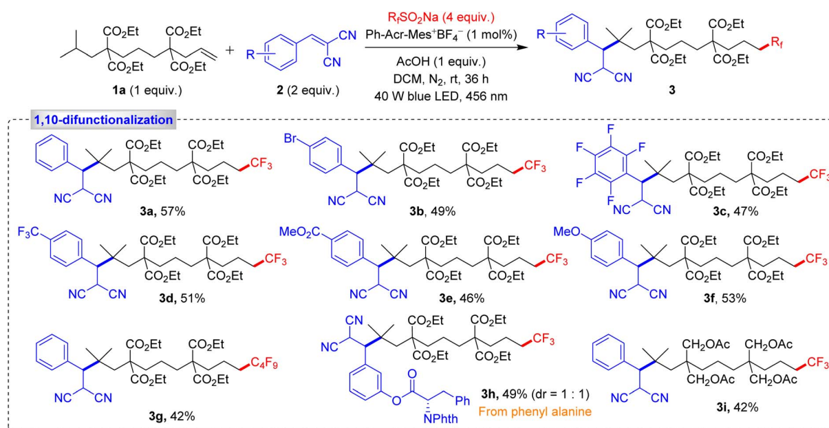
Scheme 2 Substrate scope for the 1,10-difunctionalization of alkenes. Reaction conditions: 1a (0.15 mmol, 1 equiv.), 2 (0.3 mmol, 2 equiv.), R 3 SO 2 Na (0.6 mmol, 4 equiv.), Ph-Acr-Mes + BF 4 − (1 mol%), AcOH (0.15 mmol, 1 equiv.), DCM (2.0 mL), irradiation with a 456 nm blue LED (40 W) under N 2 atm., rt, 36 h.
