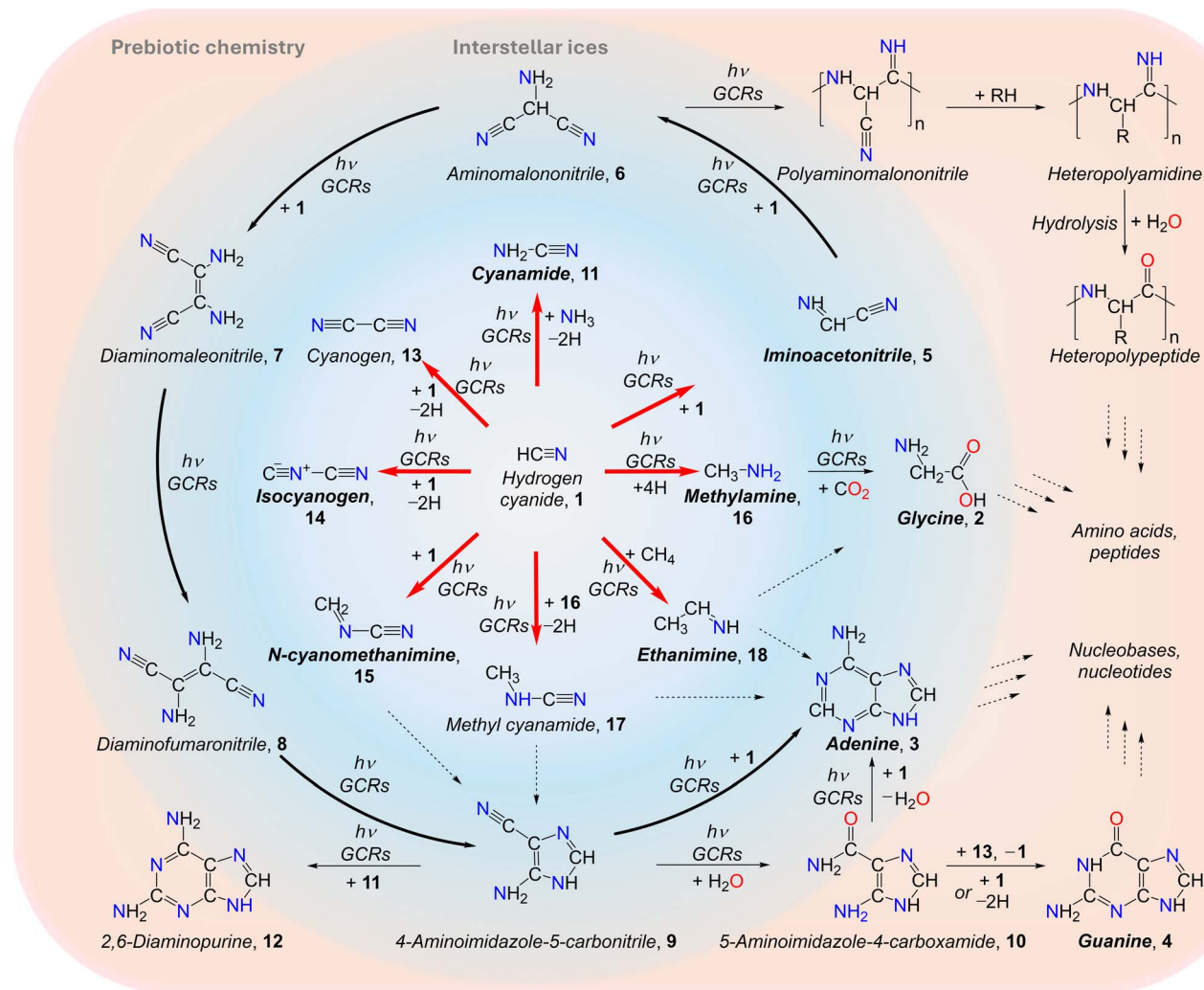
Fig. 1 Proposed formation pathways of biorelevant molecules (red arrows) in hydrogen cyanide (HCN)-containing interstellar ices and their role as precursors to biorelevant molecules such as amino acids and nucleobases. In prebiotic chemistry, hydrogen cyanide (1) plays a fundamental role in the synthesis of amino acids such as glycine (2) and nucleobases including adenine (3) (bold black arrows) and guanine (4) through non-equilibrium chemistry. Notably, 5, 11, 14–16, and 18 have been detected in the interstellar medium; 2–4 have been identified in carbonaceous asteroid Bennu and various chondrites like Murchison meteorite.
