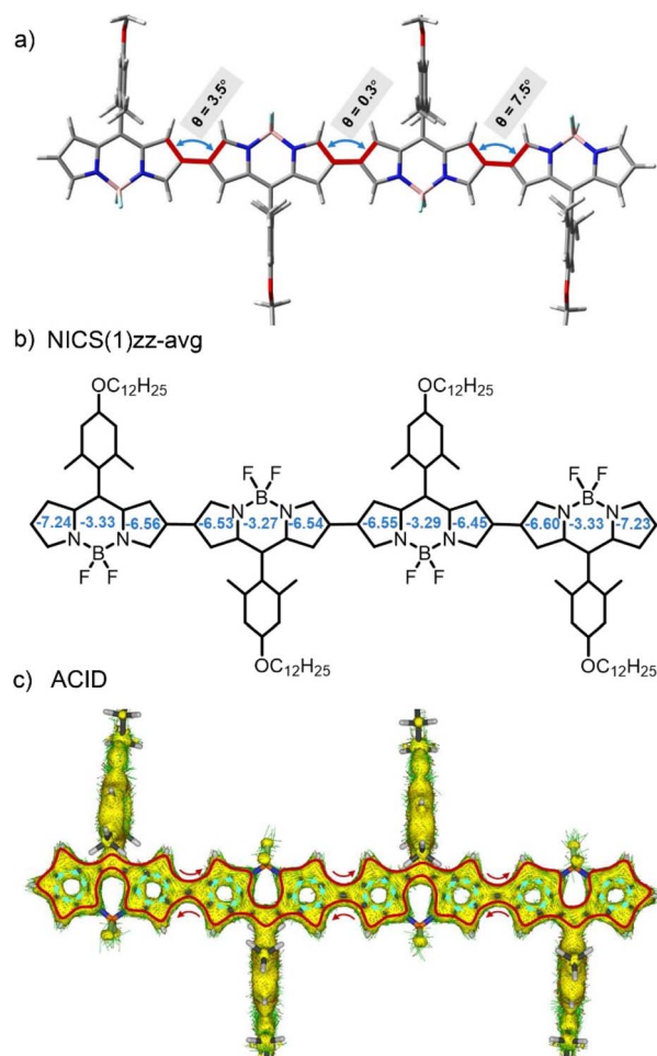
Fig. 2 (a) Optimal ground-state conformation and dihedral angles of different BODIPY units. (b) Calculated NICS(1)zz-avg values and (c) ACID plot of tetrameric BODIPY 4.
