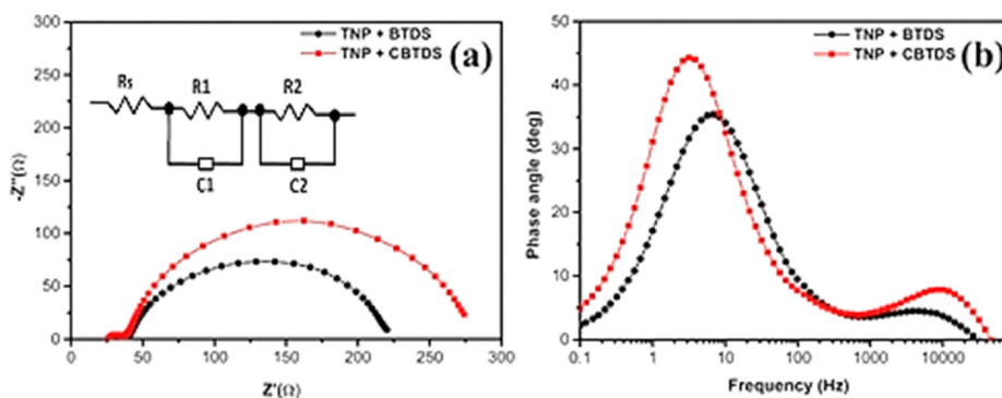
Fig. 7 Electrochemical impedance spectroscopy (EIS) of DSSCs of TNP + BTDS and TNP + CBTDS photoelectrodes at an applied potential of -0.8 V: (a) Nyquist plots with an equivalent circuit as the inset and (b) Bode plots.
