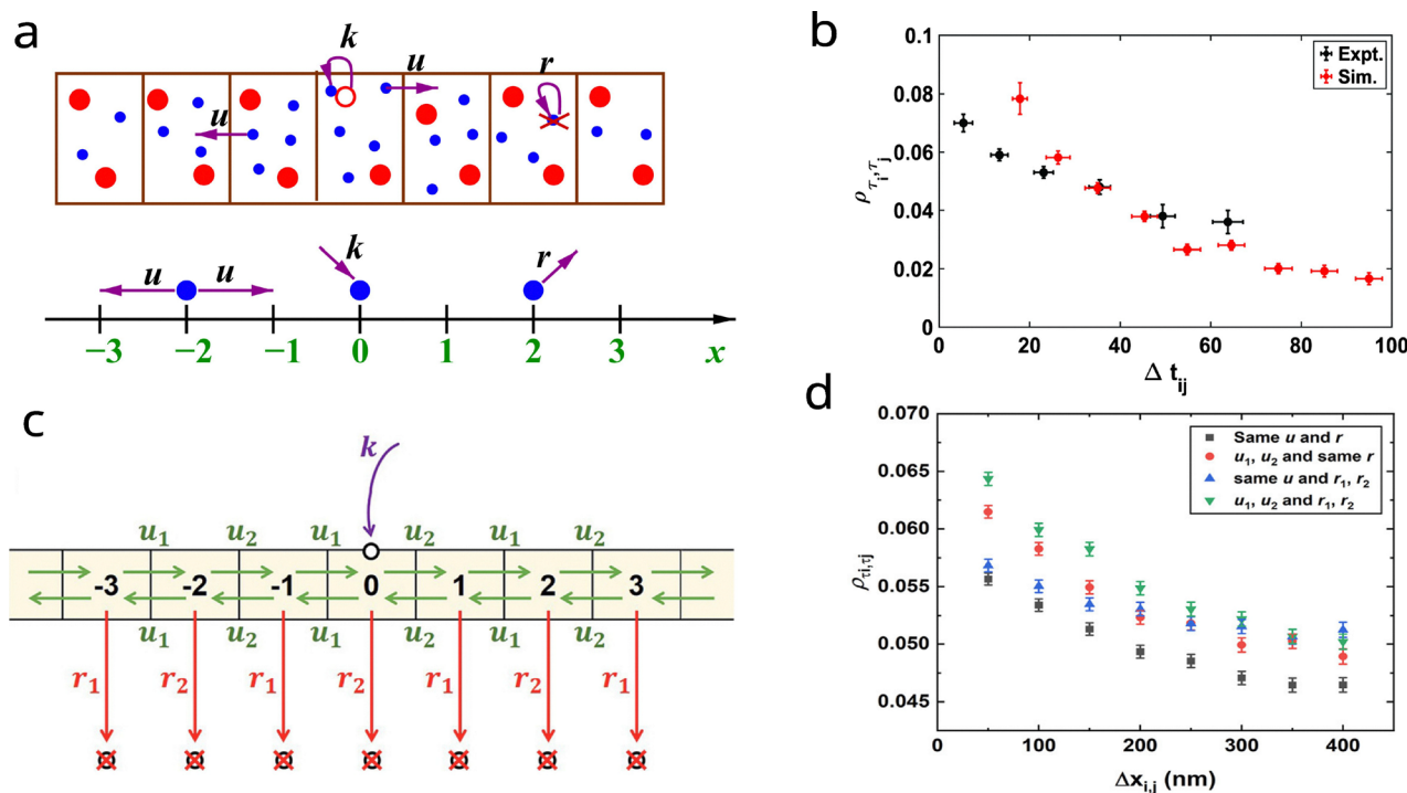
Fig. 7 Communication in the nanoparticle catalysis; (a) the schematic diagram of hole creation, migration, and disappearance on a nanorod is divided into segments of equal length. The panel at the bottom shows the discrete state model, where the lattice sites are labeled as integers for different segments. (b) Experimental and theoretical (simulated) Pearson's cross-correlation coefficients against average time separation \Delta t_{ij} of subsequent reactions at segments i and j on the Pd nanorod. (c) Model for catalytic communication with heterogeneous rate constants. (d) Pearson's cross-correlation coefficients varied with average separation \Delta x_{ij} for two segments i and j on the nanorod and comparison between heterogeneous and homogeneous cases. (a) and (b) are reproduced from ref. 158 published by PNAS under CC BY-NC-ND 4.0. (c) and (d) are reproduced with permission from ref. 143. Copyright 2023 American Chemical Society.
