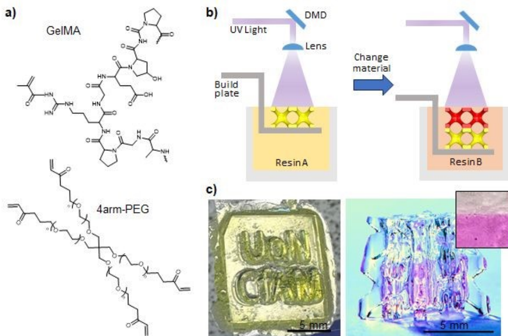
Figure 1. Hydrogel printing. (a) Chemical structure of GelMA and 4Arm-PEG-Ac. (b) Schematic illustration of high-resolution projection stereolithography (pμSLA) process for multimaterial fabrication. (c) Photographs of GelMA structure with the University of Nottingham Centre for Additive Manufacturing acronym (left) and GelMA (top) and GelMA/Rhodamine B (bottom) multimaterial structure printed into a BCC lattice structure (right), with inset showing magnified optical image of the multimaterial interface.
