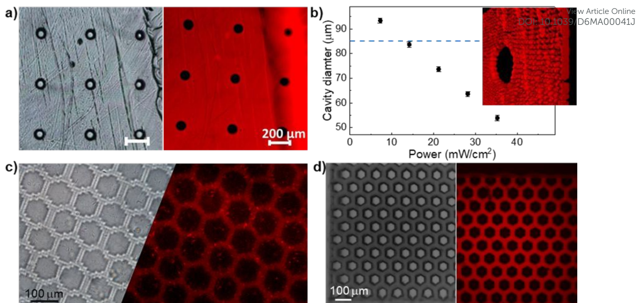
Figure 2 (a) Optical microscopy and fluorescence microscopy images of GelMA/Rhodamine B structure with cavities diameter of 85 μm and depth of 500 μm. (b) Dependence of the cavity diameter on UV power density, P , used during printing. (Inset) High resolution fluorescent image of the tilted structure ( P = 14 \text{ mW/cm}^2 ). Error bar represent standard deviation of the measured value based on at least three independent repeats. Representative optical microscopy and fluorescence microscopy images of honeycomb structures printed with GelMA 20 w/v% on (c) \mu SLA and (d) on 2PP printer.
