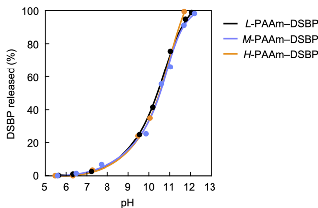
Fig. 11 Release efficiency of DSBP as a function of pH, determined from UV absorbance at \lambda = 348 \text{ nm} .
