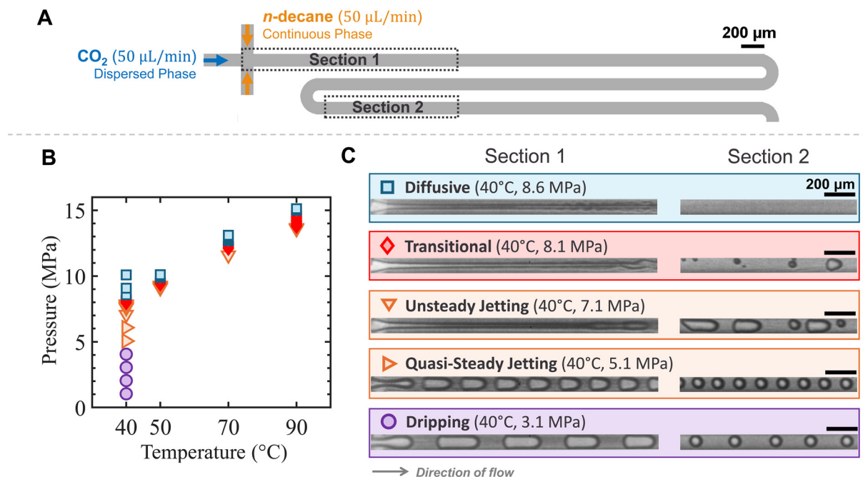
Fig. 2 (A) Microchannel schematic showing section 1 and section 2 as the regions of interest under a microscope with a 10 \times objective. \text{CO}_2 (dispersed phase) and n -decane (continuous phase) were co-injected at a constant flow rate of 50 \mu\text{L min}^{-1} at the flow-focusing junction. Section 1 captures the junction where the \text{CO}_2 -decane interface forms, while section 2 is located downstream (8.6 mm from the junction). (B) Phase diagram summarizing all the experimental conditions, showing flow regime transitions at T = 40, 50, 70 , and 90^{\circ}\text{C} . (C) Representative snapshots at T = 40^{\circ}\text{C} for each flow regime, captured from section 1 (left) and section 2 (right) as indicated in (A). Experimental conditions are noted; scale bars: 200 \mu\text{m} .
