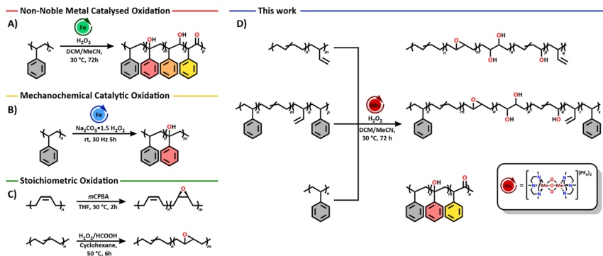
Scheme 1 (A) Non-noble metal catalysed oxidation of polystyrene. 16 (B) Solvent-free mechanochemical catalytic oxidation of polystyrene. 18 (C) Stoichiometric oxidation of polybutadiene by m\text{CPBA} and \text{H}_2\text{O}_2 /formic acid. 20,22 (D) This work on the oxidation of polystyrene and polybutadiene using a robust manganese oxidation catalyst.
