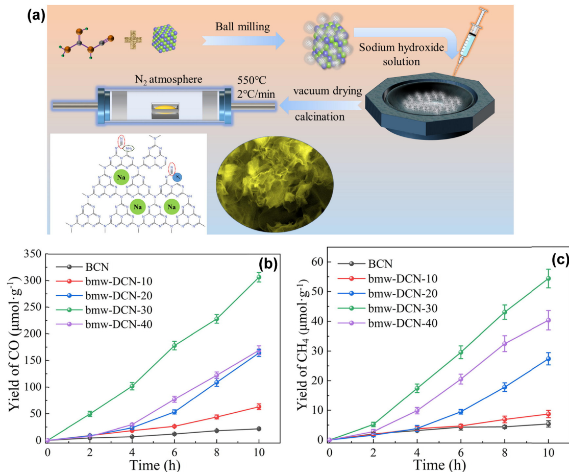
Fig. 22 (a) Diagrammatic illustration of the synthesis of Na-doped flaky g-C_3N_4 with N-defects, (b) CO and (c) CH_4 evolution rates of BCN and bmw-DCN-x. Reproduced with permission from ref. 151. Copyright 2021, Elsevier.
