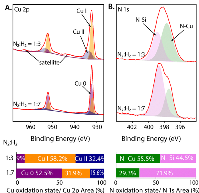
Fig. 7 XPS of particles collected on Si wafer after 10^8 pulses at 0.83 \text{ mJ pulse}^{-1} under N_2:H_2 = 1:3 or 1:7 . (A) Cu 2p with fitted Cu^0 , Cu^+ , Cu^{2+} states. (B) N 1s with N–Cu and N–Si signals. Bar plots show relative fractions.
