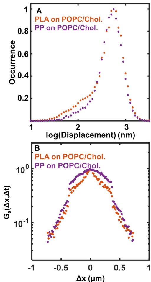
Fig. 5 Single-frame displacement and van Hove distribution of engineered PNPs on POPC lipid bilayer surface and POPC/cholesterol bilayer surface. (A) PLA and PP show one population corresponding to long displacement value for both types of surfaces. (B) PP shows a gaussian distribution indicating Brownian motion whereas PLA exhibits a central peak at the center of the distribution suggesting confined diffusion on the bilayer surface.
