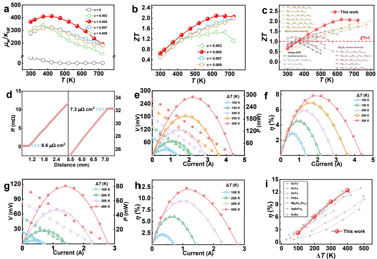
Figure 5 The thermoelectric performance of ZT and fabricated single-leg and TE module. a \mu_w/\kappa_{\text{lat}} , b ZT , c comparison of ZT values with representative n-type thermoelectric systems, including \text{Bi}_2\text{Te}_3 -, \text{Mg}_3\text{Bi}_2 - and \text{Mg}_3\text{Sb}_2 -based materials, d the measured contact resistance, e-f I - V and I - P characteristics and conversion efficiency ( \eta ) of the TE module under different temperature differences, g-h I - V and I - P curves and \eta of the single-leg generator at various temperature gradients, i comparison of conversion efficiency between this work and reported single-leg devices.
