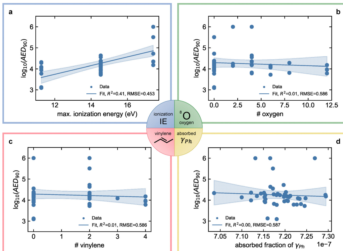
Fig. 3 Relationships between the gamma stability target AED 90 and sample properties: (a) maximum ionization energy, (b) number of oxygen atoms, (c) number of vinylene bonds, and (d) absorbed fraction of gamma photons \gamma_{Ph} . The data points are fitted by linear regression (blue line) at a 95% confidence interval (blue-shaded area).
