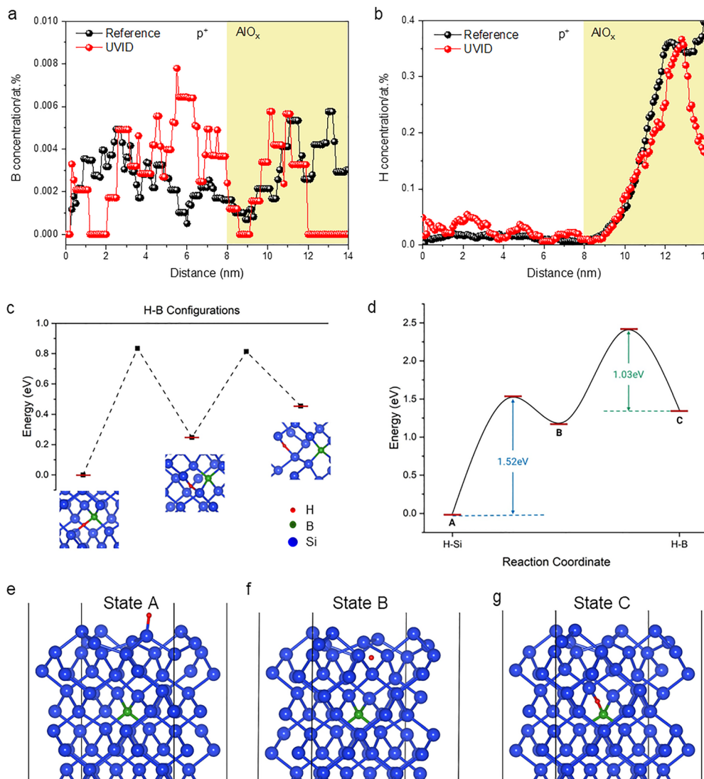
Fig. 4 1-D concentration profile of (a) B and (b) H across the interface of \text{AlO}_x and \text{p}^+ region derived from the highlighted area in Fig. S4 in reference and UVID cells (detailed in SI 4). (c) Three configurations of H-B and their relative system energies. The configuration in which H is located near the centre of the B-Si bond exhibits the lowest energy, indicating the formation of a B-H bond. (d) NEB calculation results, with states A, B and C demonstrated in (e)–(g) respectively. State A corresponds to the configuration where H passivates the Si surface by forming H-Si bonds; State B represents the intermediate state where H penetrates into the subsurface region; and State C denotes the formation of a B-H bond. The sequence A–B–C represents the UVID irradiation process, while the reverse sequence corresponds to the LSIR process.
